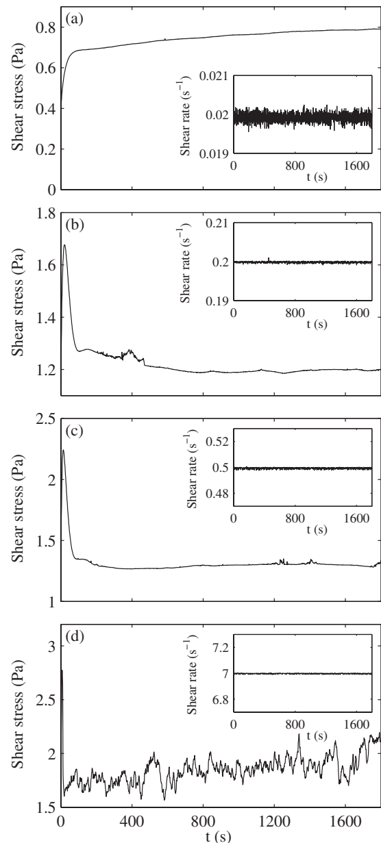
FIG. 7. Rheological time series \sigma(t) recorded at T=39.4\text{ }^\circ\text{C} for four different imposed shear rates. (a) Newtonian regime ( N ): \dot{\gamma} = 0.02\text{ s}^{-1} . (b) Wall slip regime ( S ): \dot{\gamma}=0.2\text{ s}^{-1} . (c) Shear banding regime ( B ): \dot{\gamma}=0.5\text{ s}^{-1} . (d) Unstable regime ( U ): \dot{\gamma}=7\text{ s}^{-1} . The insets show that the feedback loop of the rheometer keeps the shear rate \dot{\gamma}(t) constant to within 2% for \dot{\gamma}=0.02\text{ s}^{-1} , 0.6% for \dot{\gamma}=0.2\text{ s}^{-1} , and 0.3% for \dot{\gamma}=0.5 and 7\text{ s}^{-1} .
