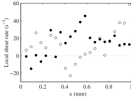
FIG. 13. Local shear rate \dot{\gamma}(x) computed from the individual velocity profiles recorded at T=39.4 °C for \dot{\gamma}=15 s ^{-1} and shown in Fig. 10.
