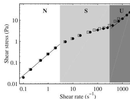
FIG. 2. Flow curve at T=37.0 °C. The full symbols ( \bullet ) correspond to the engineering data \sigma(\dot{\gamma}) while the open symbols ( \square ) represent the “true” flow curve \sigma(\dot{\gamma}_{true}) obtained once wall slip is taken into account (see text). The solid lines are \sigma=0.25\dot{\gamma} in regime (N) and \sigma=0.012\dot{\gamma} in regime (U).
