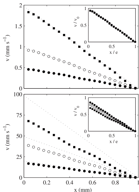
FIG. 3. Time-averaged velocity profiles at T=37.0 °C. The standard deviation is of the order of the marker size. The dotted lines are the velocity profiles expected in a Newtonian fluid without wall slip. Inset: dimensionless data v_s/v_0 vs x/e . Top: \dot{\gamma}=0.5 ( \bullet ), 1 ( \circ ), and 2 s^{-1} ( \blacksquare ). Bottom: \dot{\gamma}=20 ( \bullet ), 50 ( \circ ), and 100 s^{-1} ( \blacksquare ).
