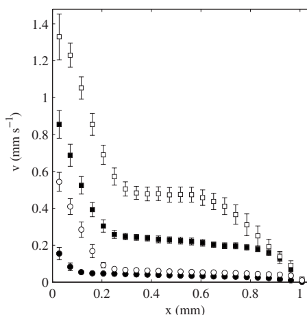
FIG. 6. Time-averaged velocity profiles at T=39.4\text{ }^\circ\text{C} in the shear banding regime noted ( B ) in Fig. 5. \dot{\gamma}=0.5 (•), 1 (◦), 1.5 (■), and 2\text{ s}^{-1} (□). The error bars correspond to the standard deviation of the measurements. Note that the corresponding slip velocities can be easily estimated from the applied shear rate and from the fluid velocity measured at the rotor using v_s = \dot{\gamma}e - v(x=0) .
