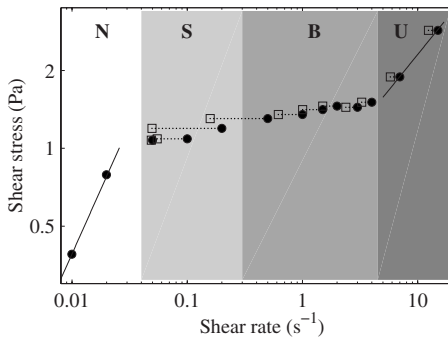
FIG. 5. Flow curve at T=39.4\text{ }^\circ\text{C} . The full symbols (•) correspond to the engineering data \sigma(\dot{\gamma}) while the open symbols (□) represent the “true” flow curve \sigma(\dot{\gamma}_{true}) obtained once wall slip is taken into account. The solid lines are \sigma=39\dot{\gamma} in regime N and \sigma=0.65\dot{\gamma}^{0.55} in regime U .
