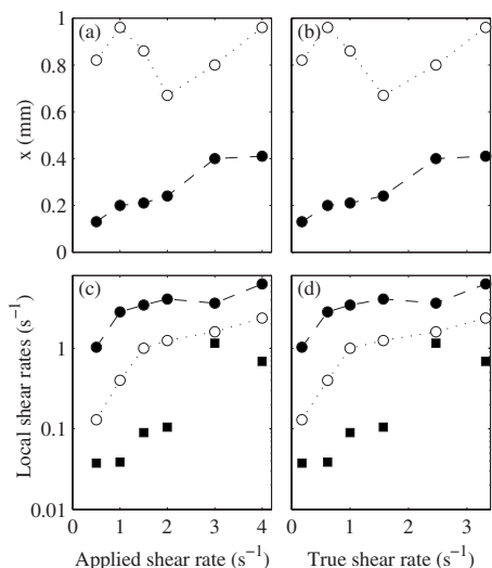
FIG. 9. Analysis of the three-band velocity profiles recorded in regime (B) at T = 39.4\text{ }^\circ\text{C} . Positions of the interfaces inside the gap as a function (a) of the applied shear rate and (b) of the true shear rate. Local shear rates in the highly sheared bands at the rotor ( \bullet ) and at the stator ( \circ ) and in the central weakly sheared band ( \blacksquare ) as a function (c) of the applied shear rate and (d) of the true shear rate.
