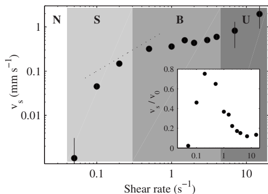
FIG. 8. Time-averaged slip velocity v_s at the rotor at T = 39.4\text{ }^\circ\text{C} vs applied shear rate \dot{\gamma} . The error bars correspond to the standard deviation of the measurements. The dashed line is v_s = v_0 . Inset: relative slip v_s/v_0 at the rotor vs applied shear rate \dot{\gamma} .
