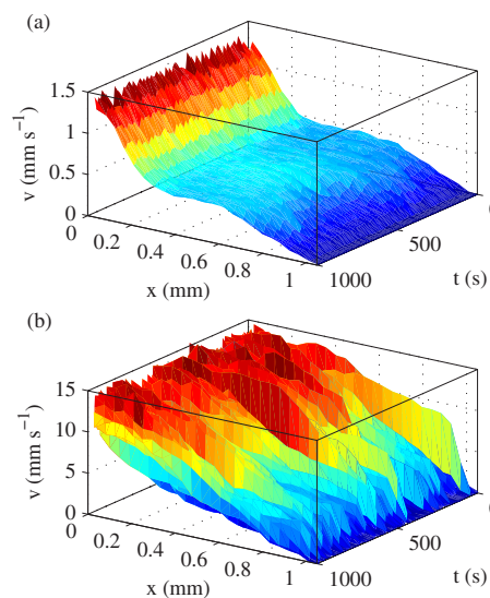
FIG. 11. (Color online) Spatio-temporal representation of the velocity profiles v(x, t) at T = 39.4\text{ }^\circ\text{C} for (a) \dot{\gamma} = 2\text{ s}^{-1} and (b) \dot{\gamma} = 15\text{ s}^{-1} .
